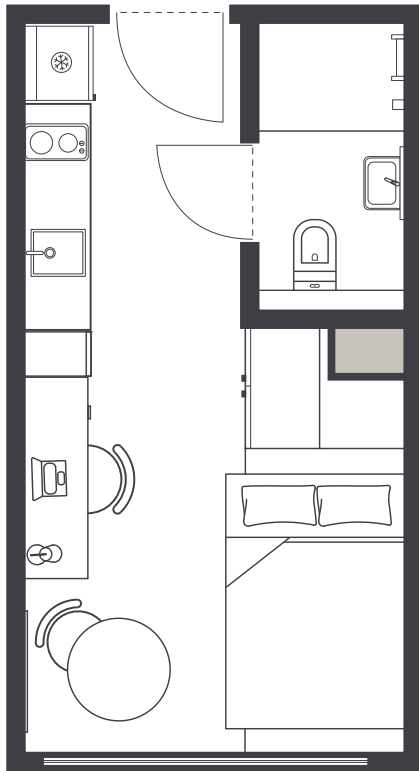
LAYOUT 1
